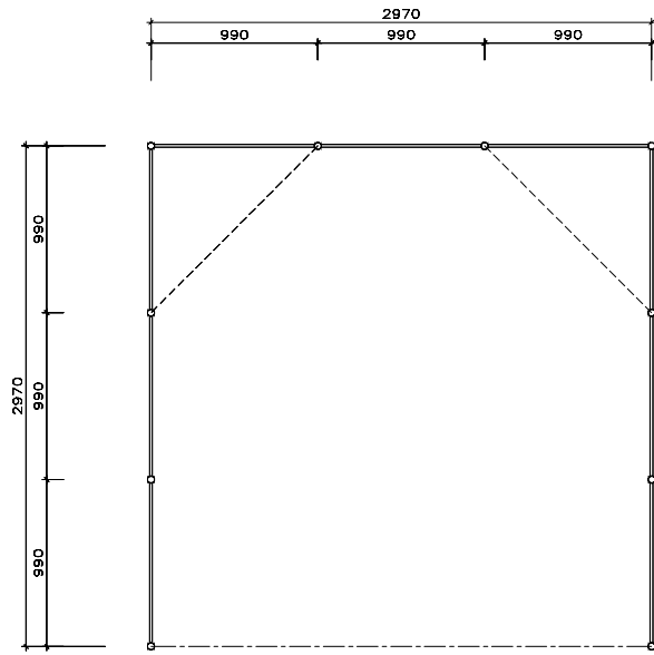
Floor Plan
