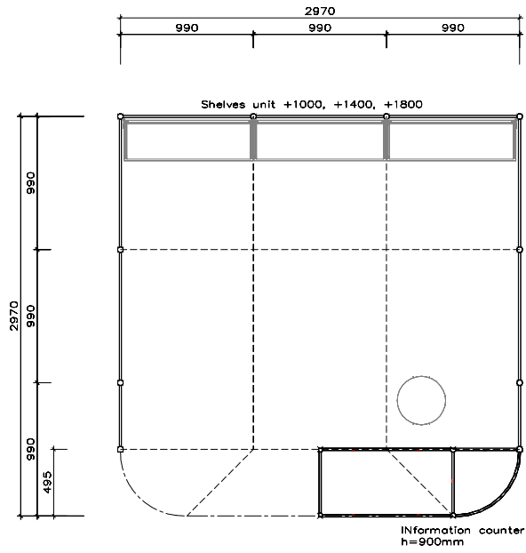
Floor Plan
