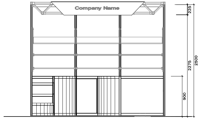
Elevation Plan
